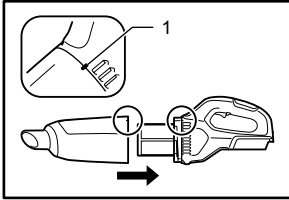
1. Alignment marks
